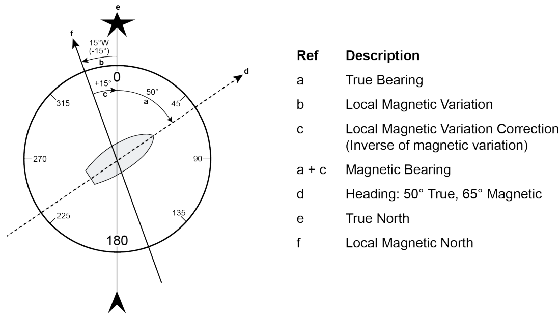
Figure 5: Illustration of Magnetic Variation and Correction
